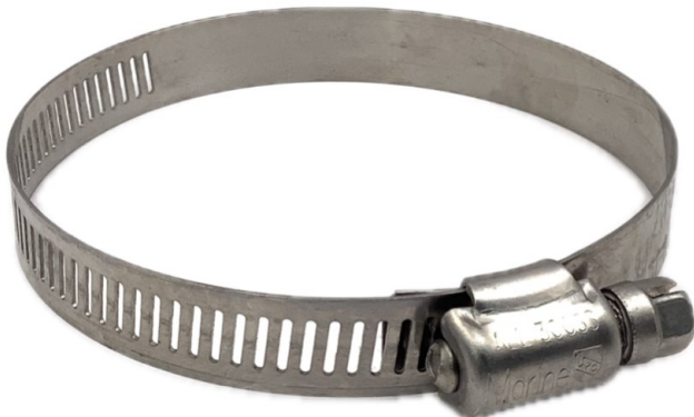
424-2044 #44 HOSE CLAMP S/S 1/2" WIDE 2-1/4-3-1/4" (57-82MM) DIA.
