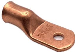
737-0064 2/0 AWG 1/4 HOLE COPPER LUG
