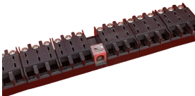
764-0016 18 CIRCUIT ATO FUSE BLOCK-1/2 BUSSED
