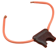
763-0016 12 AWG ATO FUSE INLINE HOLDER NO COVER
